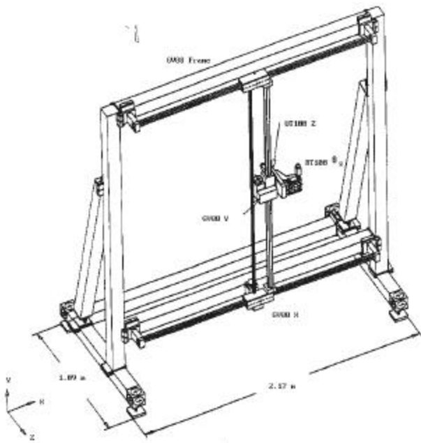
Figure 4 NSI 255 scanner isometric
