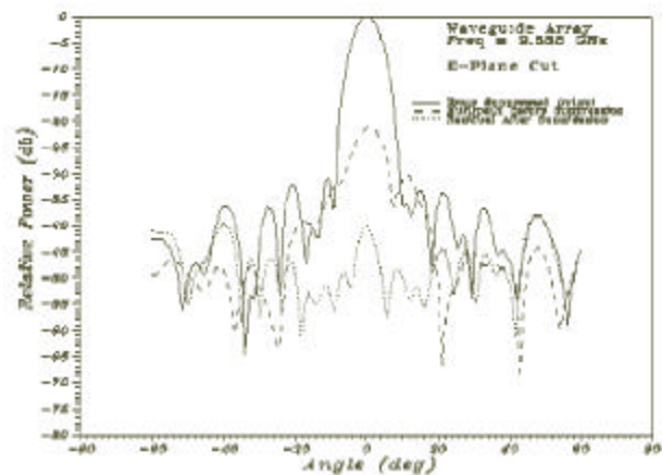
Figure 5 Multipath suppression
