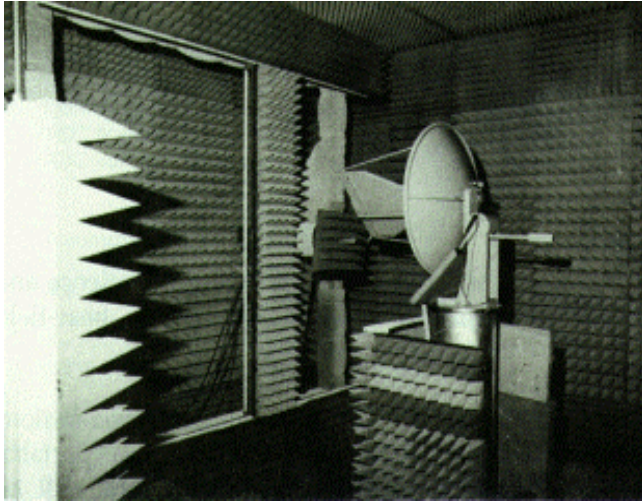
Figure 1 NSI 5' By 5' Planar/Cylindrical Near-Field System
