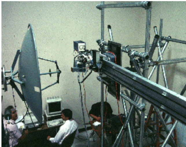
Figure 2 12' Diameter Plane-Polar System
