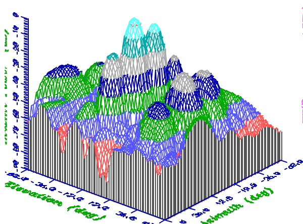
Figure 3 Anechoic Chamber Reflections
