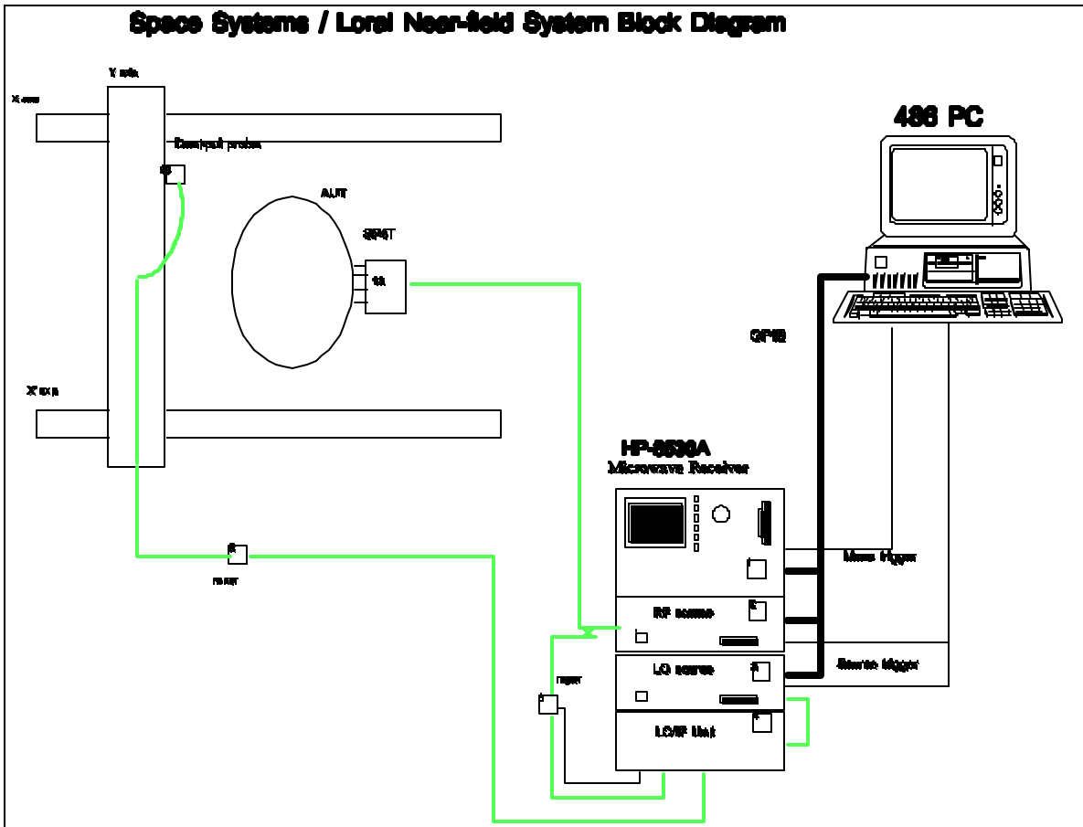
Figure 5 - SS/L RF Sub-system Block Diagram
