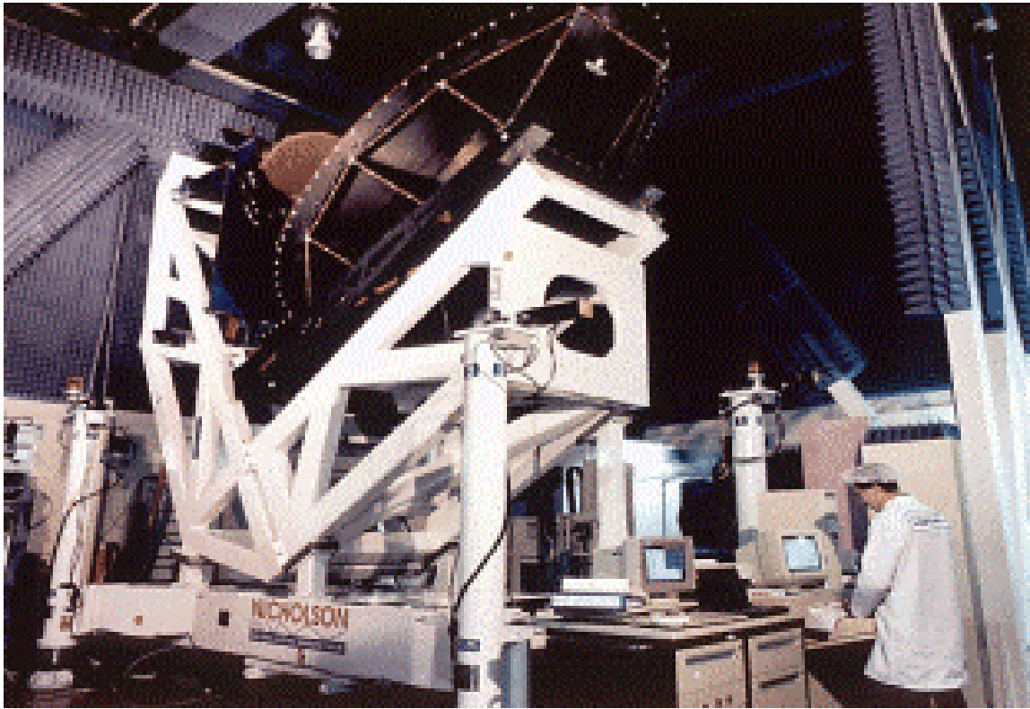
Figure 3 - NSI Scanner Testing SS/L Antenna
