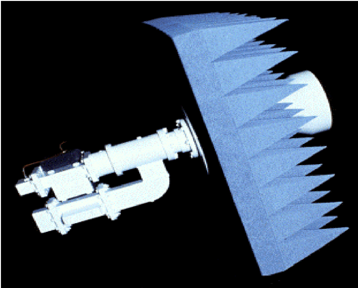
Figure 4 - Dual-Polarization Probe Assembly
