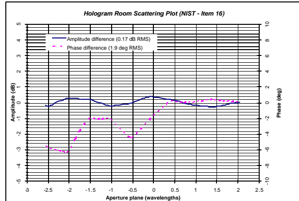
Figure 6 Room Scattering Error Plot
