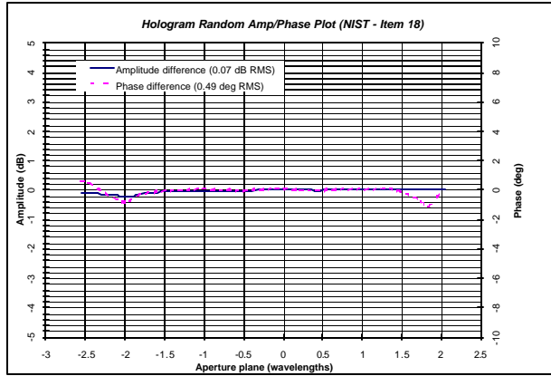
Figure 4 Random Amplitude and Phase Error Plot
