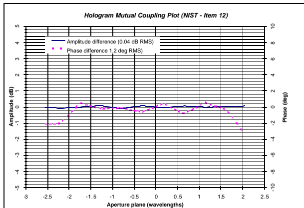
Figure 5 Mutual Coupling Error Plot
