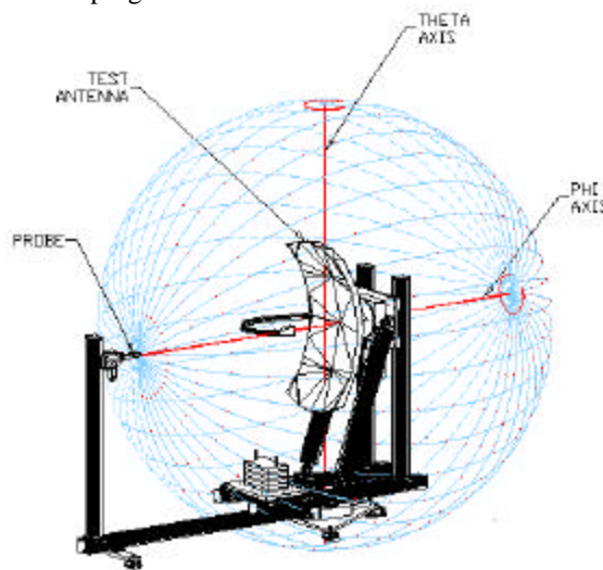
Figure 1 Spherical Measurement System
