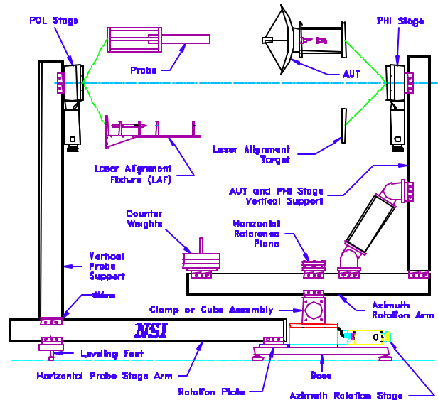
Figure 6 Spherical System Alignment Diagram
