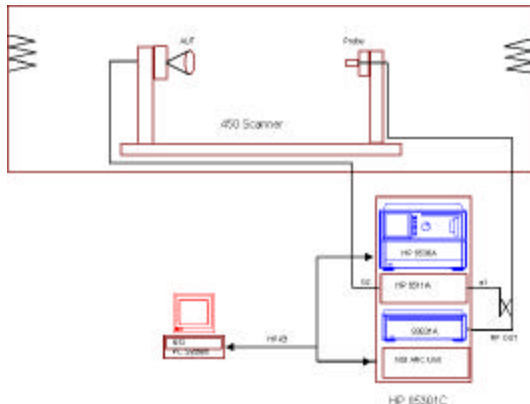
Figure 3 - RF Subsystem Block Diagram
