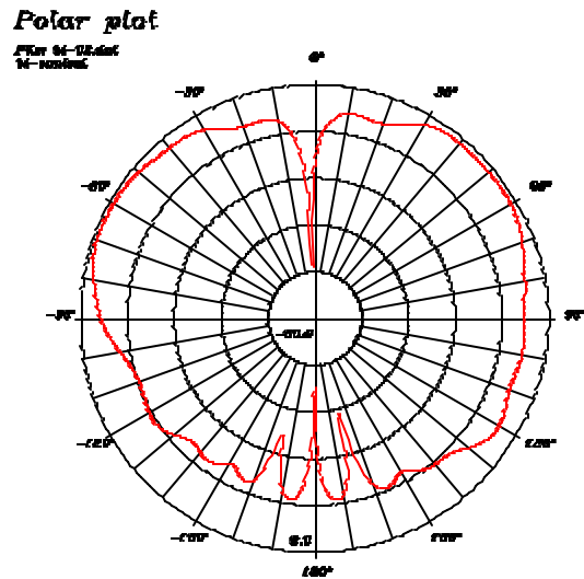
Figure 9 Broadbeam Bi-Conical Antenna Pattern
