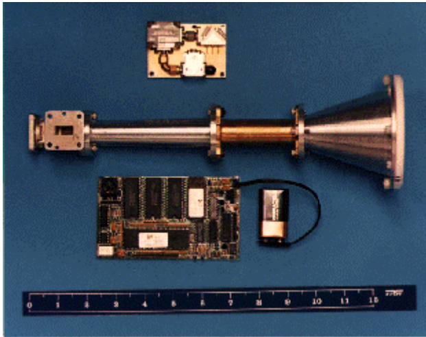
Figure 4 - HHMR Components
